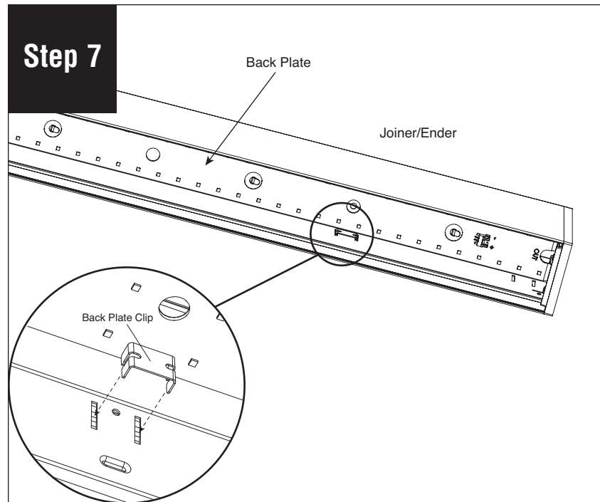
Replace back plate at end of luminaire by holding it in the original position and pushing the clips back in.
