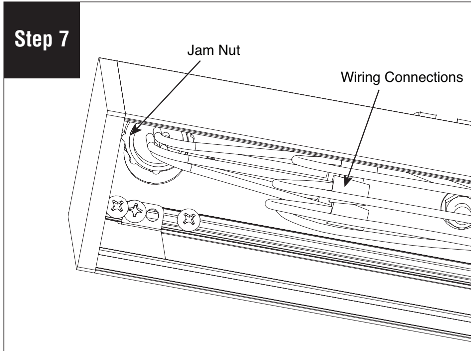
Make wiring connections.
