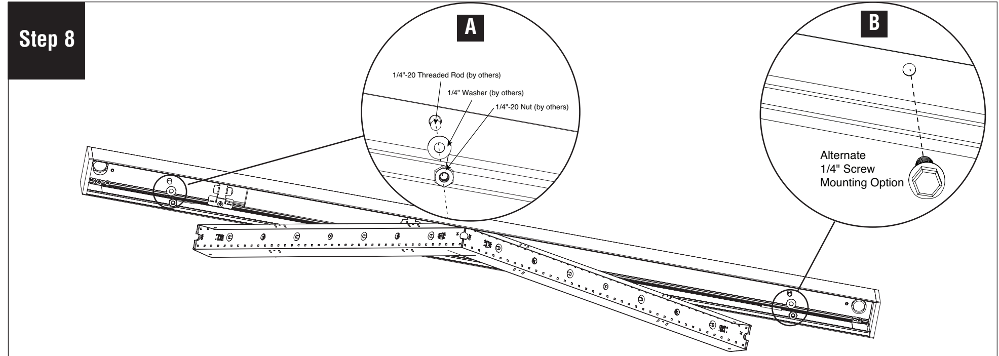
A. Install 1/4" washers (by others) and 1/4"-20 nuts (by others) onto 1/4"-20 threaded rod (by others). B. Alternate mounting option - Install 1/4" screw (by others) through mounting hole into proper structurally supported blocking (by others).
