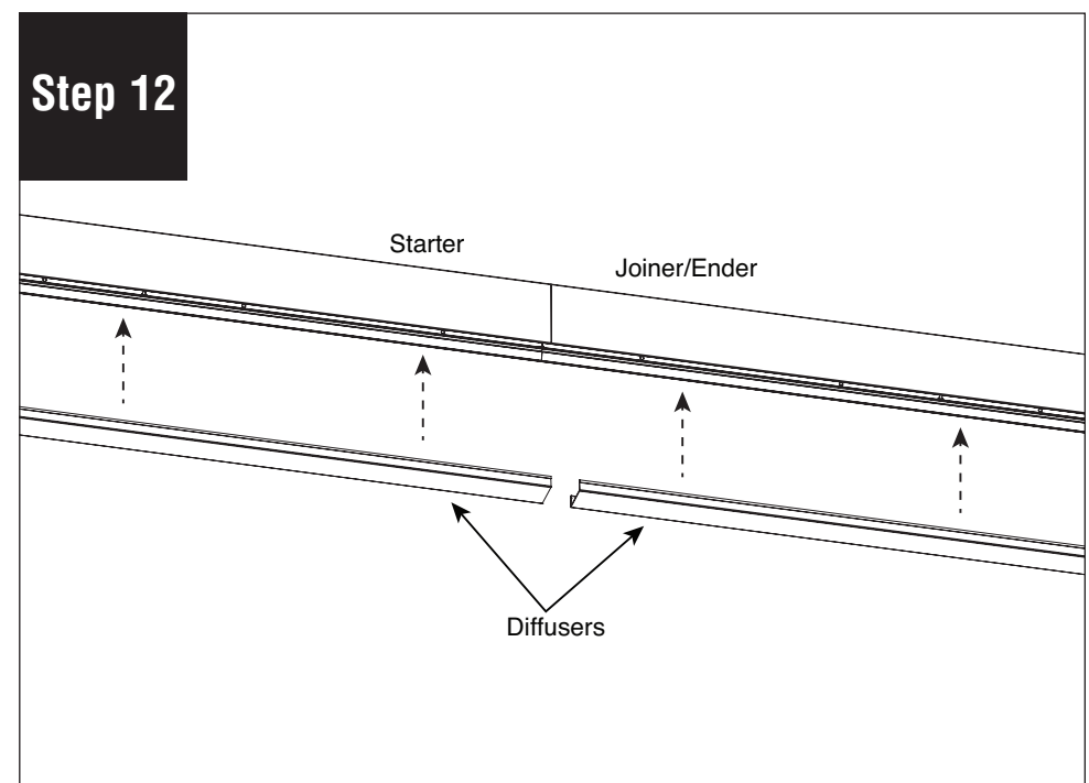
Reinstall diffusers and turn power on to luminaire.
