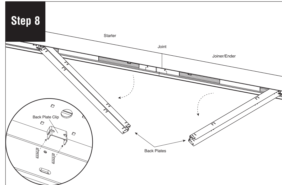
Remove back plate clips at the joint of both luminaires and slowly swing down back plates.
