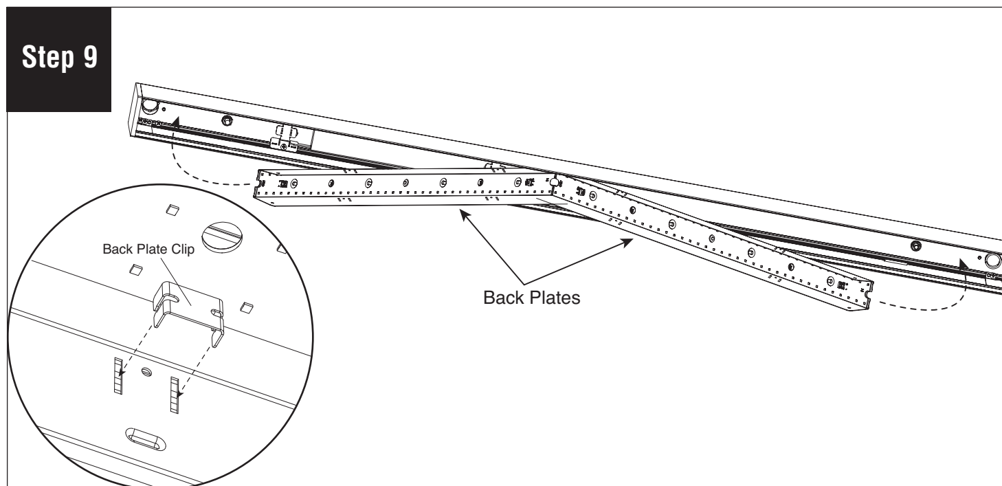
Replace back plates by holding them in their original position and pushing the clips back in. Make sure wire connections are not pinched. (If 1 ft. back plate assembly is near joint, reconnect feed harness to LED board).
