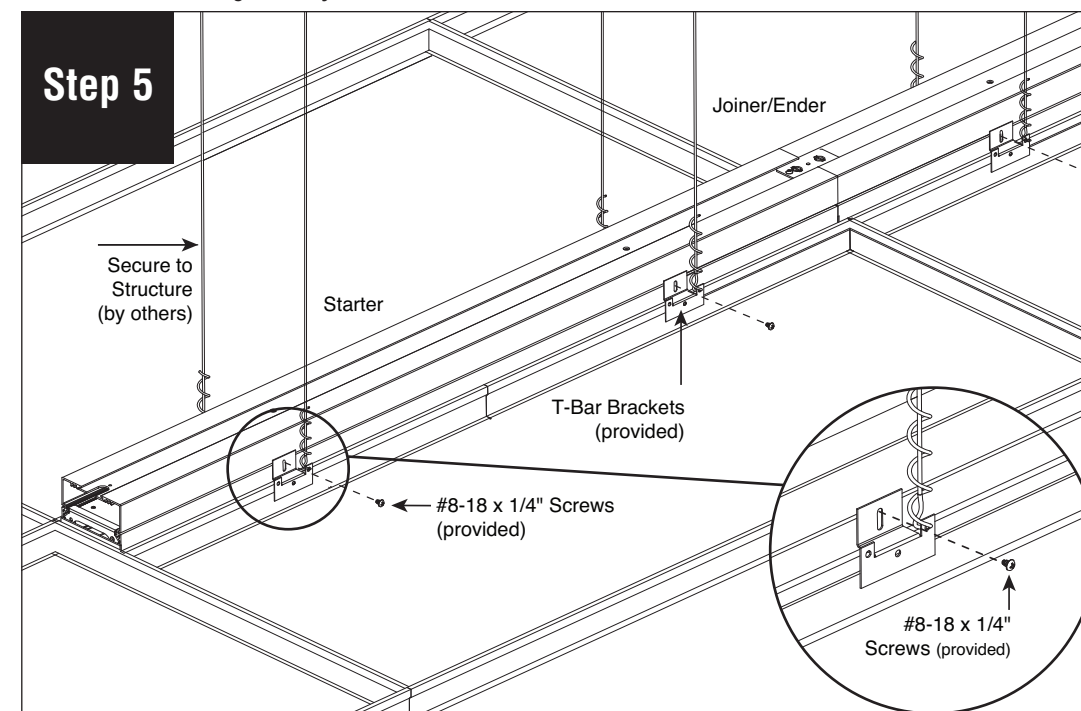
Use #8-18 x 1/4" screws (provided) to install brackets on all luminaires. Secure all luminaires to building structure using tie-wire, as per code.
