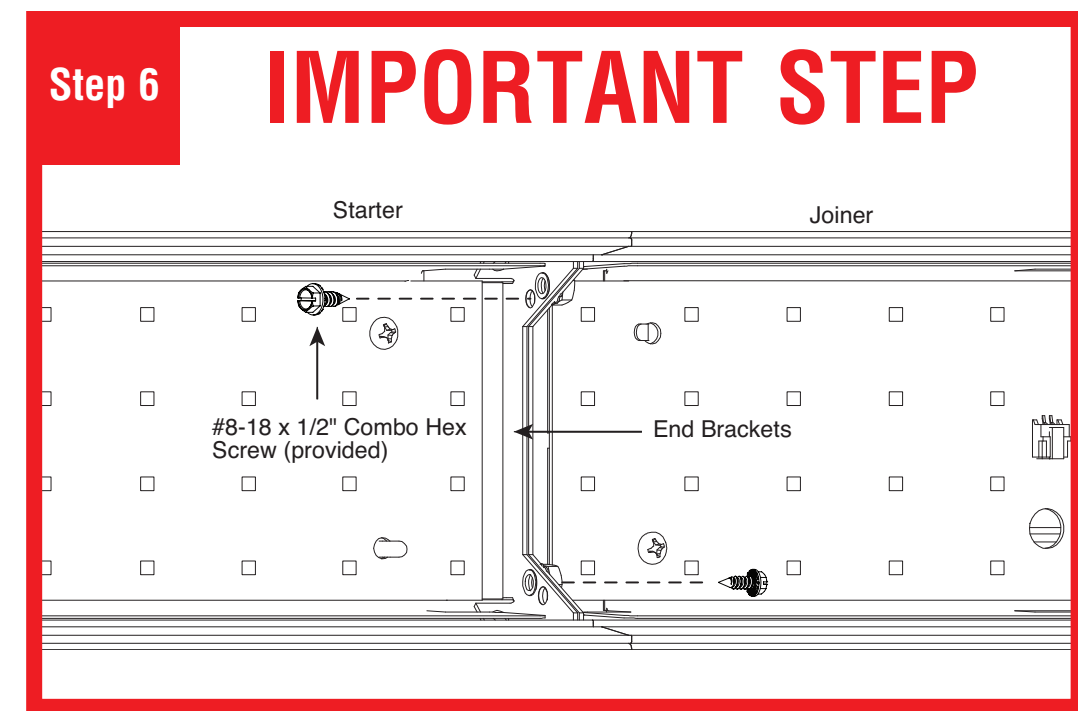
IMPORTANT STEP: Install the two #8-18 x 1/2" combo hex screws (provided) into end bracket as shown. Screws can be installed from the left or right. When installed correctly these hex screws will pull luminaires together to make a tight joint. CAUTION: Do not over-tighten.
